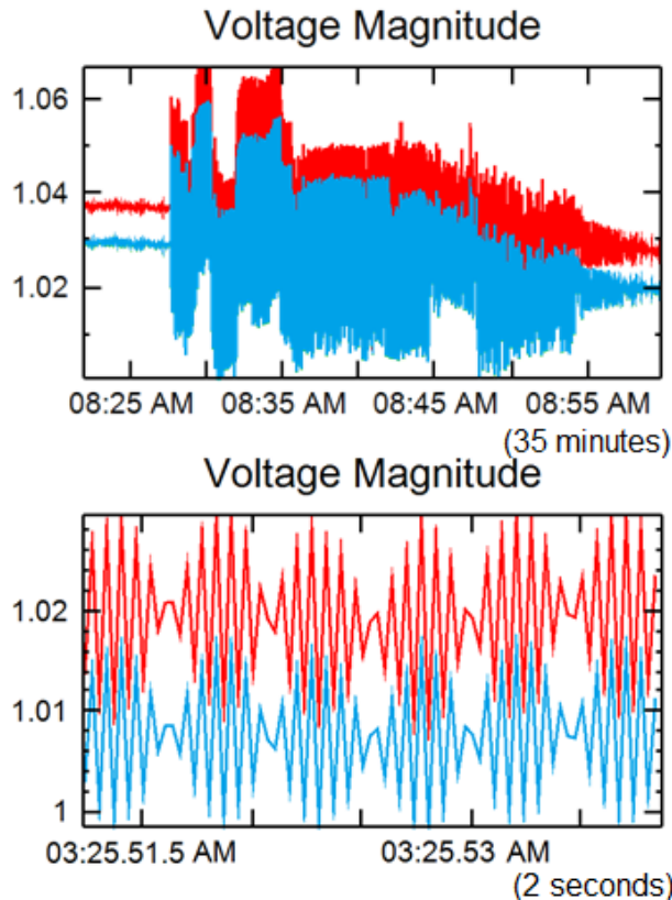
Figure 13 – Windfarm Oscillations
