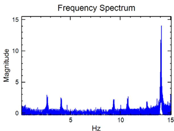
Figure 11 – FFT Detection shows undesirable oscillations at 14Hz.
