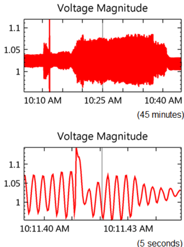
Figure 16 – New 3Hz Wind Farm Oscillation Event
