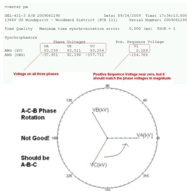
Figure 18 – Phasing error discovered during commissioning
