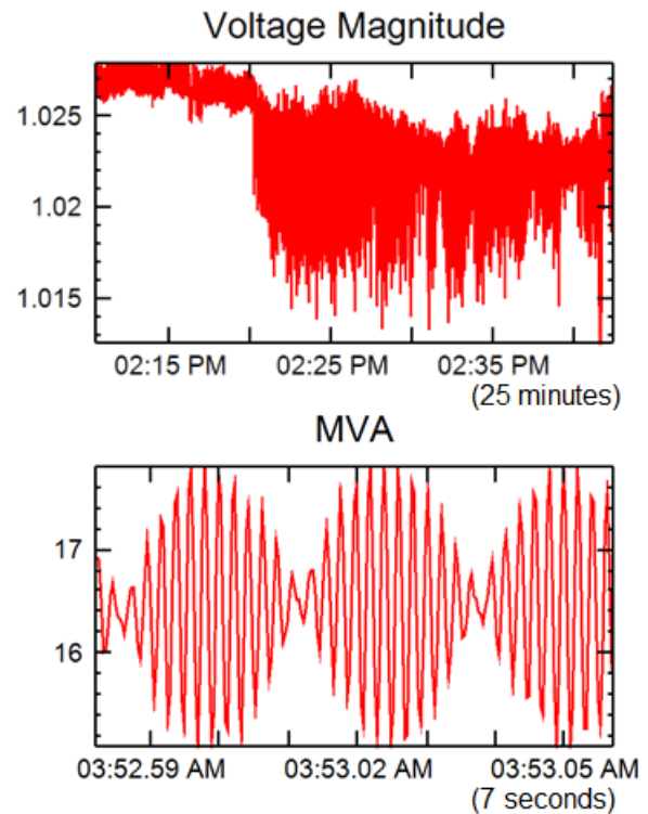
Figure 19 – Monitoring Power Quality
