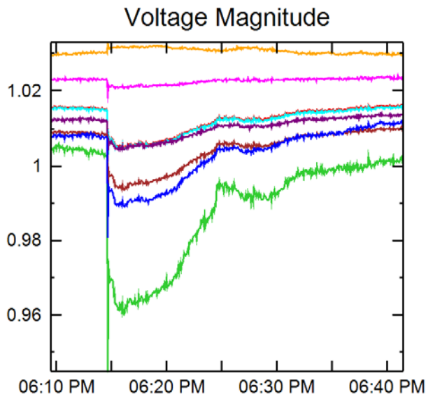
Figure 6 – Voltage Recovery Assessment
