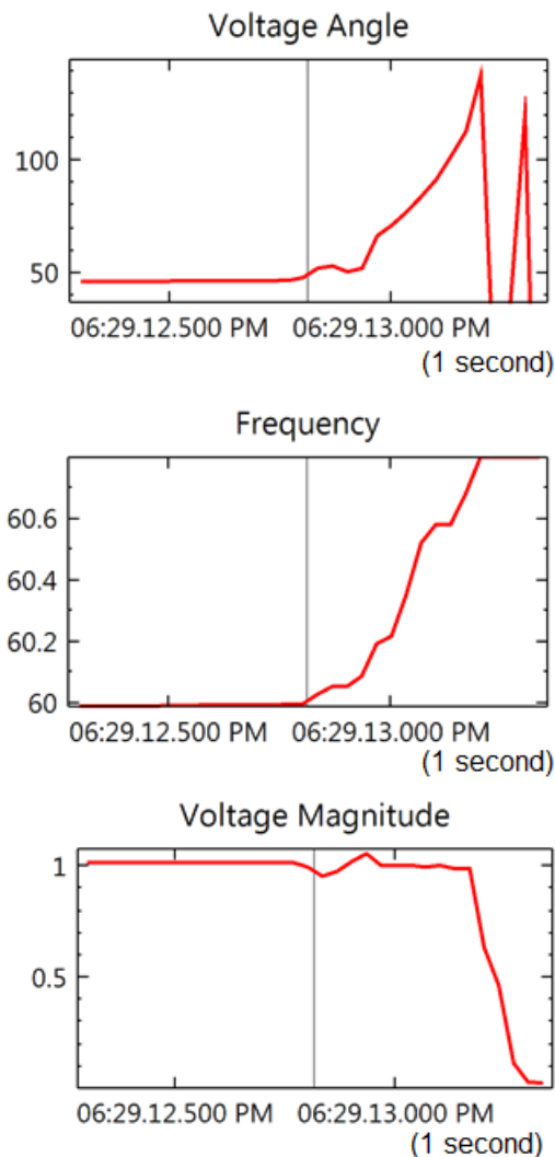
Figure 25 – 138kV South 4th St – Imo Line Trips
