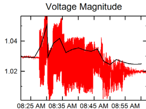
Figure 15 – Comparison of PMU and SCADA data
