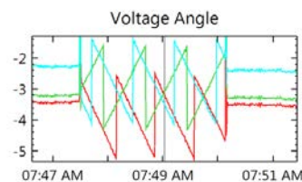
Figure 10 – Interference from a close RF source can jam GPS reception
