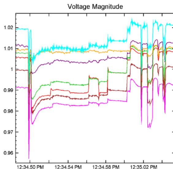
Figure 5 – Ten Second Fault Event Shows System Stress
