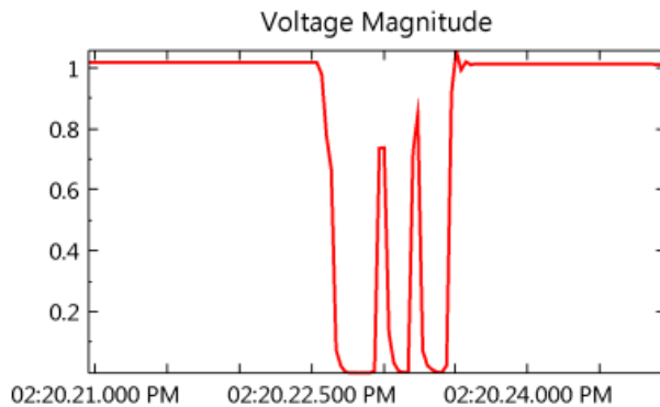
Figure 9 – Failed reclosing attempt due to incorrect settings
