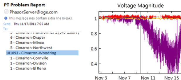
Figure 8 – PT Problem report shows a failing analog input
