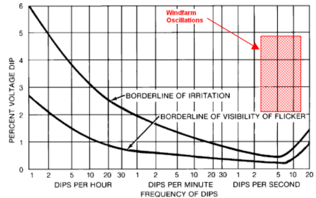
Figure 14 – Flicker region of Windfarm Oscillations
