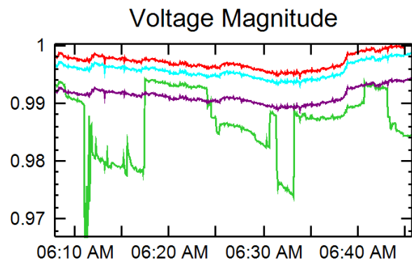
Figure 7 – Loose PT connection discovered
