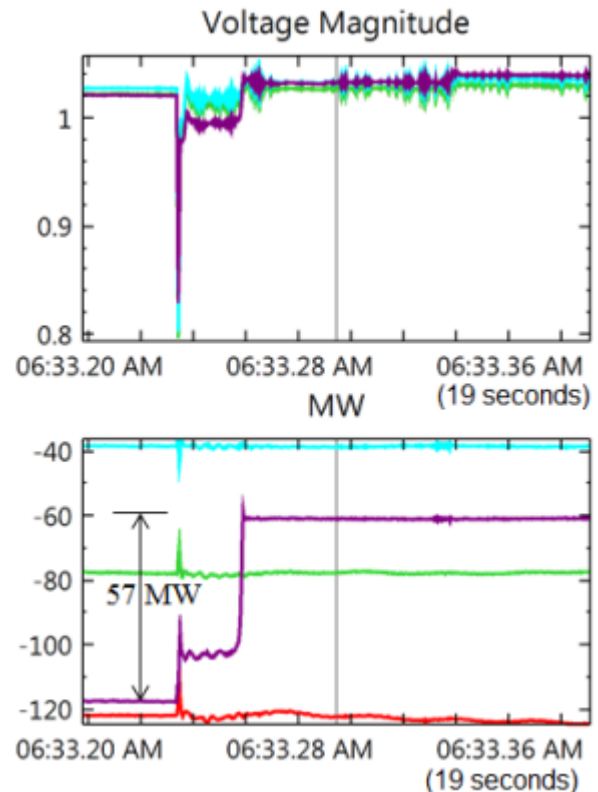
Figure 17 – Monitor Wind Farm Low Voltage Ride Through
