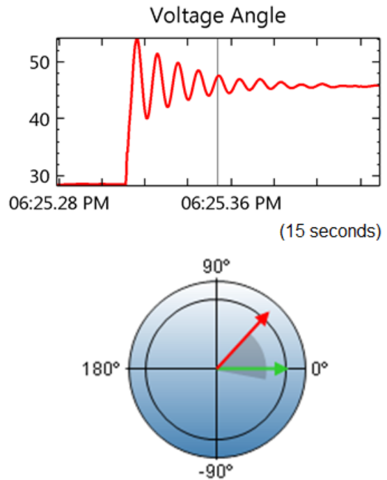
Figure 24 - Dewey - El Reno Line Trips
