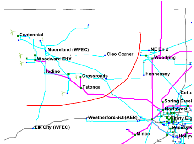
Figure 21 – Transmission Map of Northwest Oklahoma
