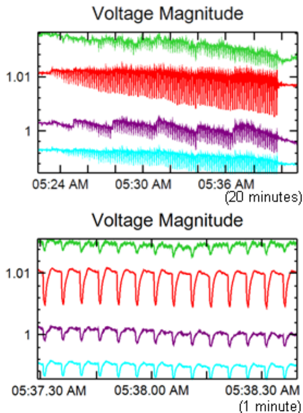
Figure 12 – Generation Unit Oscillations
