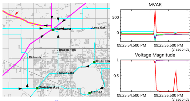
Figure 3 – Fault Location Using VAR Flows
