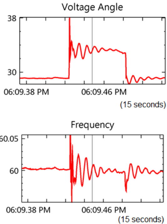
Figure 23 – 138kV Dewey-Woodward Line Trips
