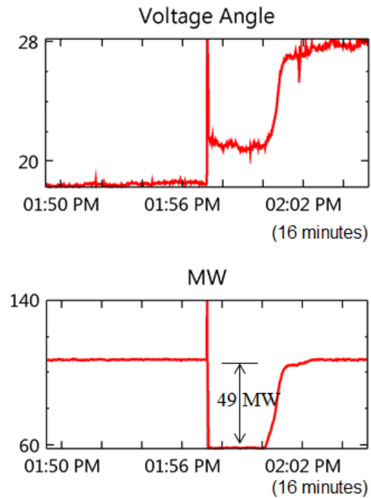
Figure 22 – 345kV Tatonga Line Trips
