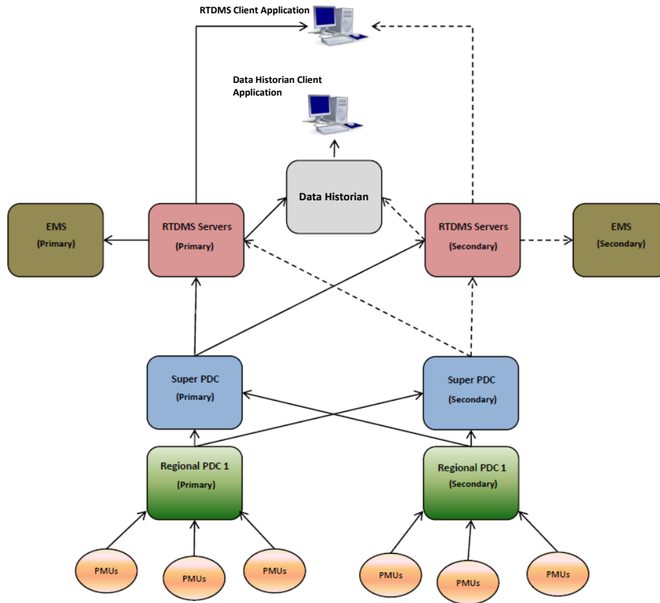
Figure 8. Synchrophasor Data Flow Diagram (Provided by Duke Energy Carolinas)
