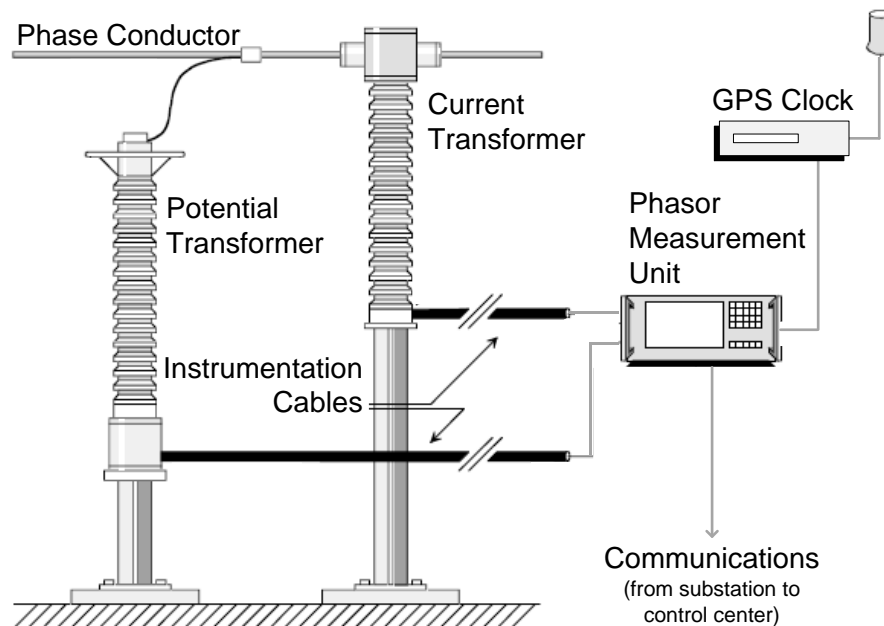
Figure 7. Example Synchrophasor System Installation within a Substation
